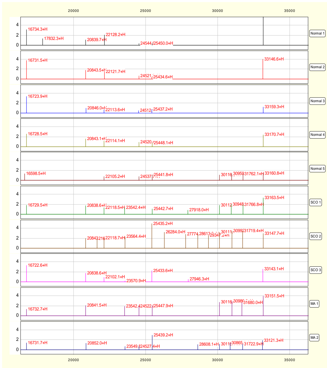
Figure 4. SELDI profiling performed by using hydrophobic chips ( H_4 ) to compare and identify differences in the protein expression patterns between human testis with normal and abnormal spermatogenesis at the molecular weight from 1.6 to 3.6 kDa (i.e., using SPA as a matrix).
